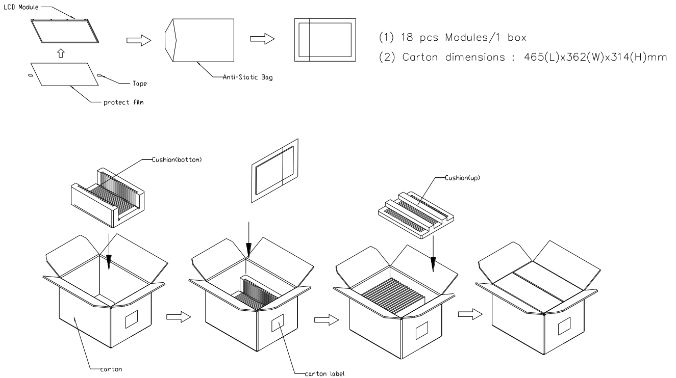
Figure. 9-1 Packing method
